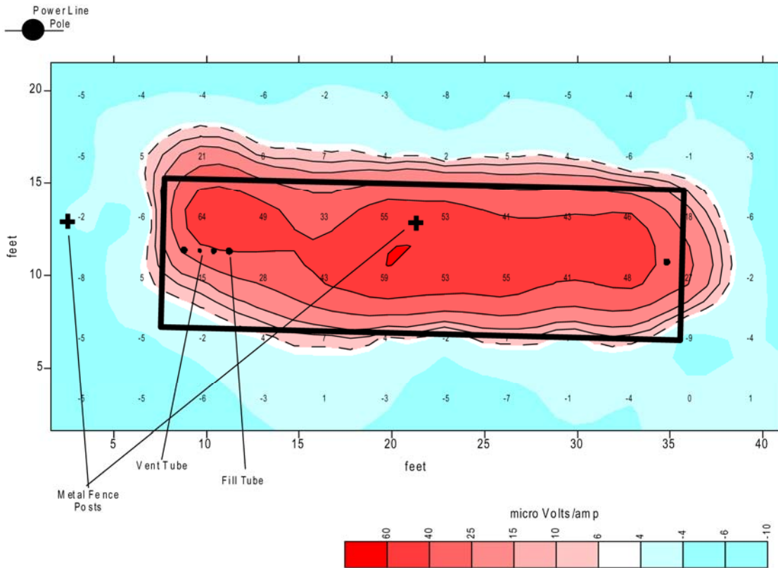
Figure 4: Plan view map of NanoTEM data, window 28, normalized. The values shown are microvolts, plotted at the center of each 1 meter receiver loop. The dark rectangle outlines the actual location of the tank.
